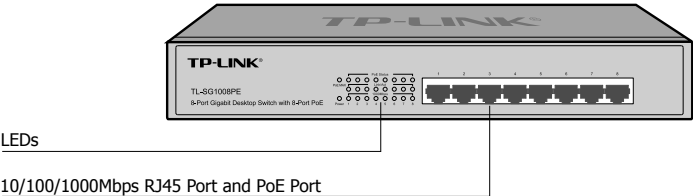
Figure 1-7 Front Panel of TL-SG1008PE
