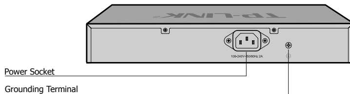
Figure 1-12 Rear Panel of TL-SG1008PE
