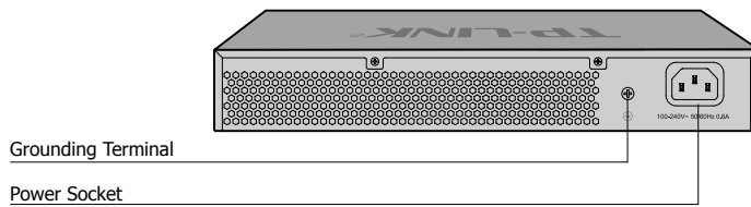
Figure 1-10 Rear Panel of TL-SG1024D/TL-SG1016D
